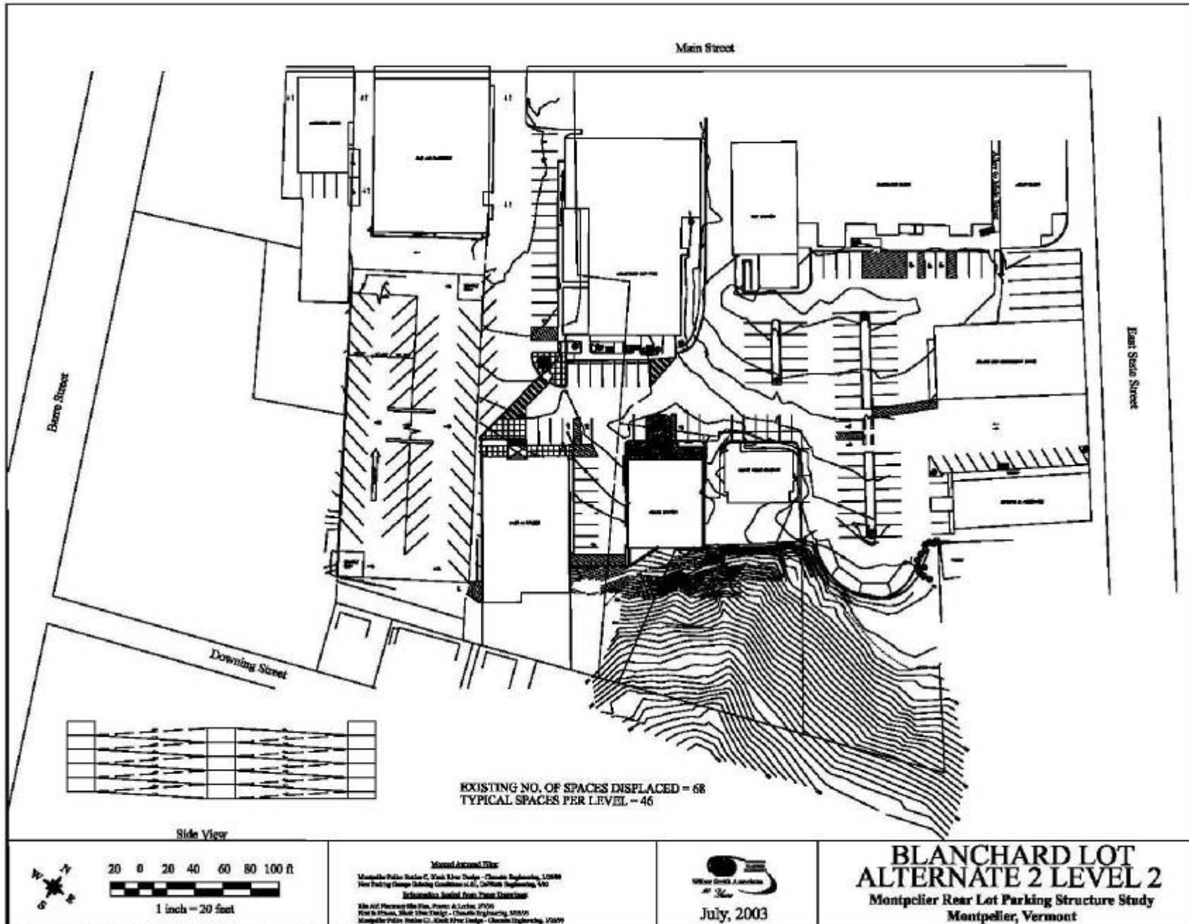
Figure 7 BLANCHARD LOT ALTERNATE 2 – LEVEL 2 Montpelier City Hall Rear Lot Parking Study City of Montpelier
